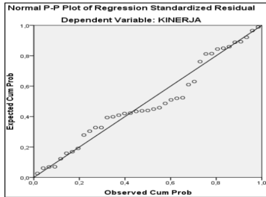
Gambar 2. Sebaran residual data
