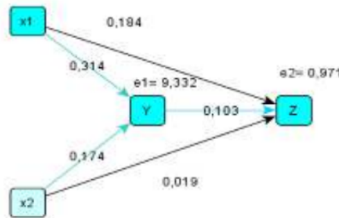
Gambar Diagram Jalur Model 2
