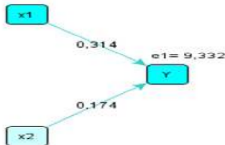
Gambar Diagram jalur model I
